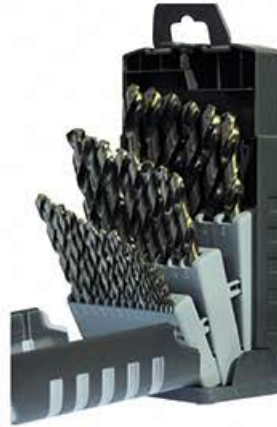
29PCS TWIST DRILL SET Size(inch):1/16-1/2 × 1/64
